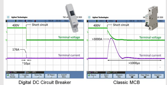
400V DC short circuit disconnection performance benchmarking
